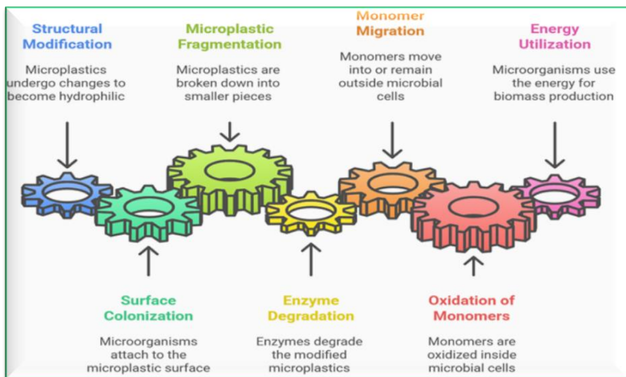
Fig. 6. Bioremediation pathway of microplastic (adapted from Ali et al., 2024).
