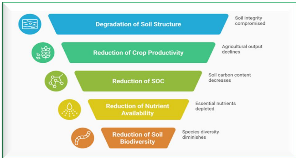
Fig. 1. Different degradation processes in soil due to microplastic pollution (adapted from FAO and UNEP 2021).
